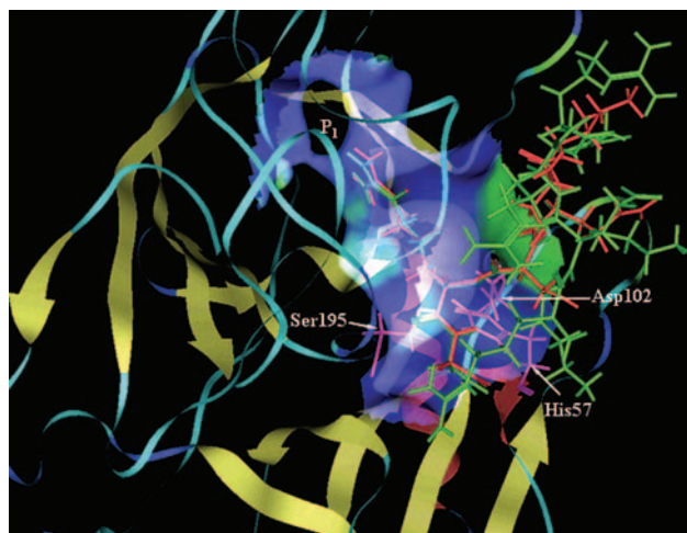
Fig. 1. The complex structures are obtained by docking peptides to trypsin. Trypsin is rendered in ribbon drawing, the nonapeptide RERRRKRR↓G is in green stick drawing, and the hexapeptide SIQSR↓G is in red stick drawing. The hydrophobic and hydrophilic surfaces of the S 1 pocket are colored in green and blue, respectively (for interpretation of the references to color in this figure legend, the reader is referred to the web version of this paper)
